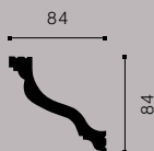
WT17 WALLSTYL®
