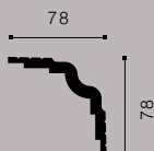
WT3 WALLSTYL®
